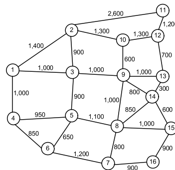
Fig. (2): Sample network
